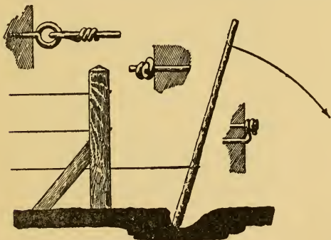
Fig. 58.—Stretching wire fencing
